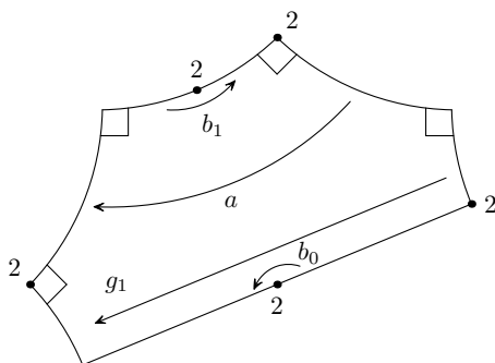
FIGURE 6. (0; 2, 2, 2, 2) , g_1 = SUS^3
