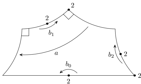
FIGURE 5. (0; 2, 2, 2, 2)
